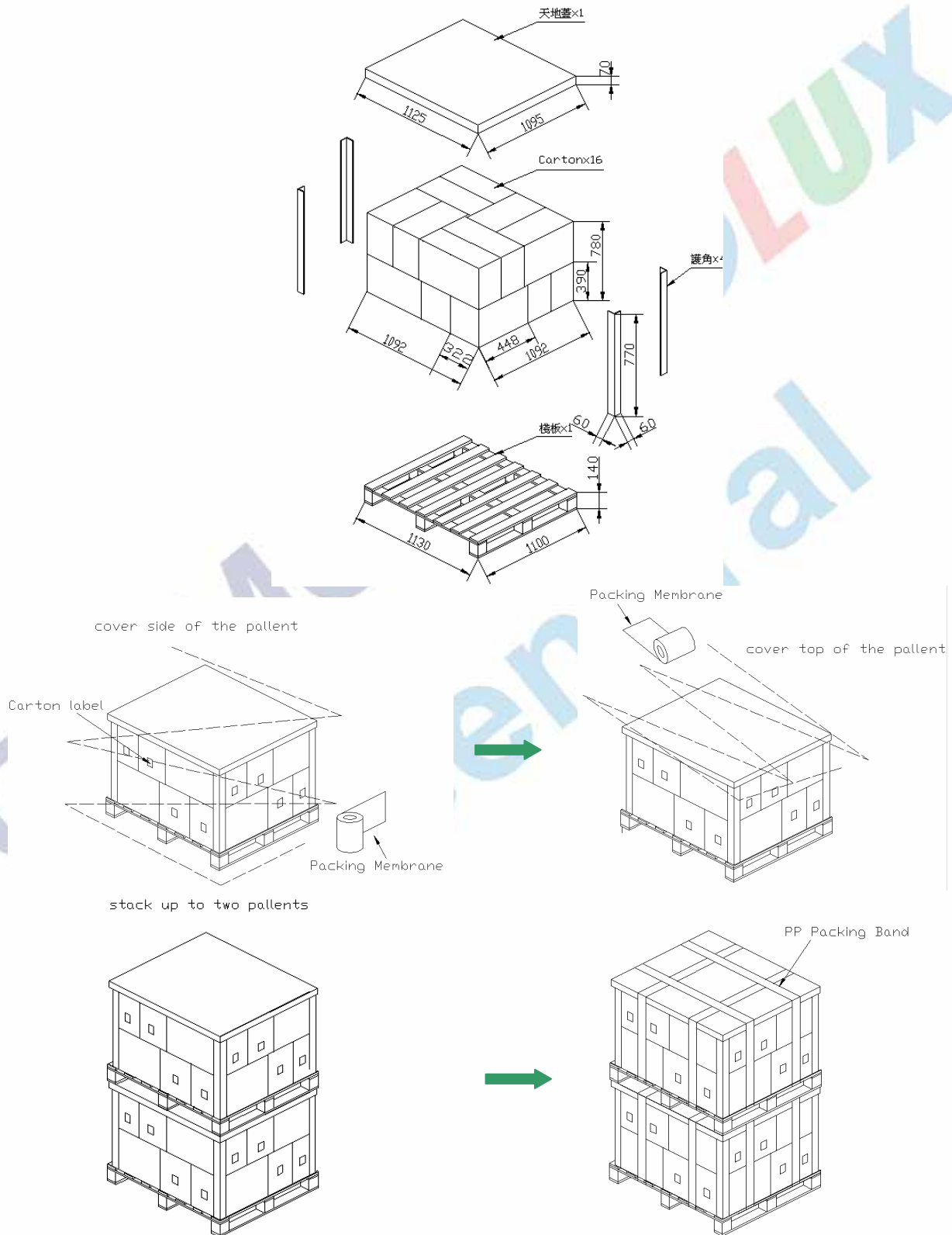
Figure. 7-2 Packing method
